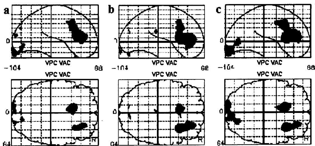
FIG. 1. Brain maps of retrieval mode. Sagittal (upper) and transverse (lower) projections of brain regions were significantly more activated in the recognition conditions than in the reading condition. (a) Meaning-Read, (b) Voice-Read, (c) New-Read.
